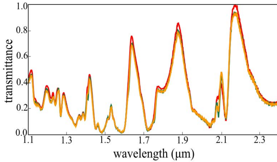
Figure 3 Transmission through the PhC slab measured at normal incidence as a function of wavelength, with the electric field aligned along the \Gamma -X direction ( \varphi = 0^\circ , red trace), along an intermediate direction ( \varphi = 22.5^\circ , green), and along the \Gamma -M direction ( \varphi = 45^\circ , orange).
