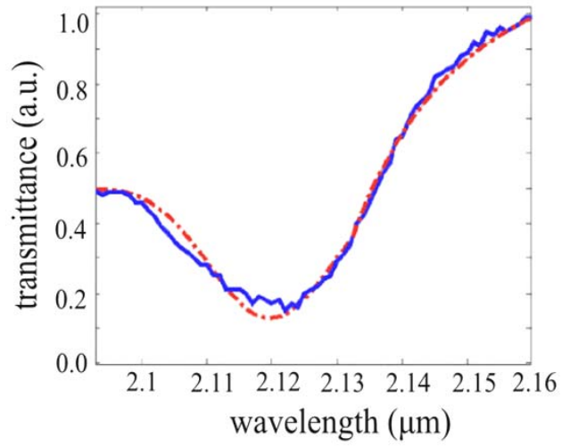
Figure 5 Example of a measured transmission spectrum (solid blue trace) fitted with the superposition of a Lorentz and Airy function (Fano-Airy function, dash-dotted red trace). The fit yields a Q-value of 125 for the Lorentzian component.
