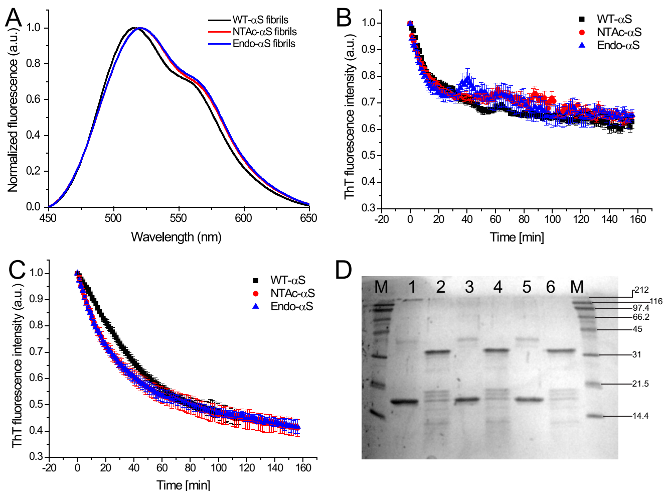
FIGURE 8. A , fluorescence emission spectra of FE-dye bound to \alpha S fibrils. 20 \mu M WT- \alpha S (black), NTAc- \alpha S (red), and Endo- \alpha S fibrils (blue) were incubated for 1 h with 2 \mu M FE-dye in PBS buffer at room temperature. The fluorescence emission spectra were acquired using an excitation wavelength of 420 nm and excitation/emission slit widths at 5 nm. B , stability of \alpha S fibrils to urea exposure followed by ThT fluorescence. Comparable fibril denaturation rates and loss of \beta -sheet content were observed for WT- \alpha S and the acetylated protein fibrils. C , proteinase K digestion assay wherein the \beta -sheet content of the fibril solution was followed by ThT fluorescence. The data points in panels B and C represent mean \pm S.D. of a minimum 3 independent measurements. D , the corresponding Coomassie-stained SDS-PAGE (12%) gel. Standard molecular weight markers (lane M) are shown on the right side of the gel. Undigested \alpha S fibrils were loaded in lanes 1 (WT- \alpha S), 3 (NTAc- \alpha S), and 5 (Endo- \alpha S), whereas proteinase K-digested fibrils after completion of experiment were loaded in lanes 2 (WT- \alpha S), 4 (NTAc- \alpha S), and 6 (Endo- \alpha S).
