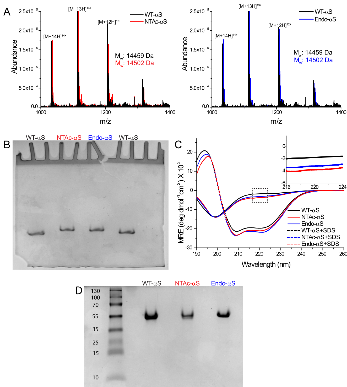
FIGURE 1. Biochemical characterization of \alpha S variants. A, ESI-MS data of purified monomeric WT- \alpha S, NTAc- \alpha S, and Endo- \alpha S, respectively. All samples were prepared in 10 mM ammonium acetate buffer with the concentration of \alpha S monomers kept constant at 15 \mu M. For a given m/z value, the corresponding charge state is indicated. Molecular masses ( M_r ) were calculated as follows: m/z value = [M + xH]^{x+} . M_r = (m/z \text{ value} \times x) - x . B, acetic acid gel electrophoresis data of monomeric WT- \alpha S, NTAc- \alpha S, and Endo- \alpha S. 5 \mu M of each protein sample was loaded into gels and as shown above, the relative migration of WT- \alpha S was more than that of acetylated- \alpha S, which migrated at similar positions. C, CD spectra showing the conformational transition from a random coil to a \alpha -helix upon the addition of SDS micelles. The inset shows the slightly higher absorbance of acetylated- \alpha S at 222 nm compared with WT- \alpha S. All data obtained with WT- \alpha S are depicted with black, with NTAc- \alpha S with red, and Endo- \alpha S with blue colors, respectively. D, native-PAGE gel of WT- \alpha S, NTAc- \alpha S, and Endo- \alpha S showing absence of any higher ordered aggregates in either sample. A standard PageRuler™ Plus pre-stained protein ladder was loaded in the left-most lane and the numbers correspond to molecular masses in kDa. A minute band appears in the WT- \alpha S lane very close to the beginning of the resolving gel, which is larger than 250 kDa in size.
