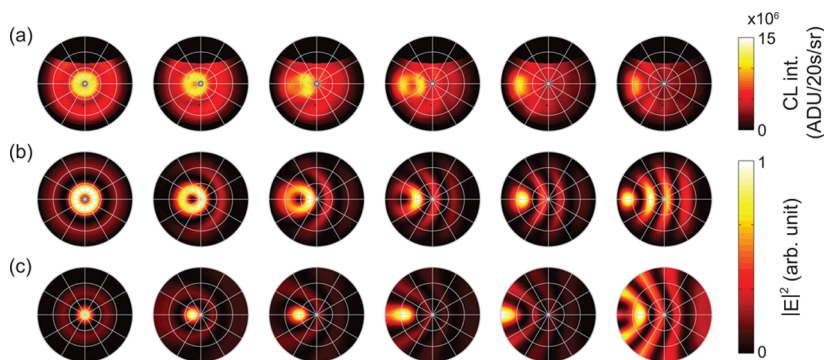
Figure 9. (a) Measured radiation pattern as a function of excitation position for a typical patch antenna ( d = 1.3 \mu\text{m} , \lambda = 700 \text{ nm} ). Calculated radiation patterns from (b) radially polarized dipole model and (c) scalar model. From left to right: e-beam excitation position at the center of the disk to the right mid-edge ( x = r/2 ) of the disk.
