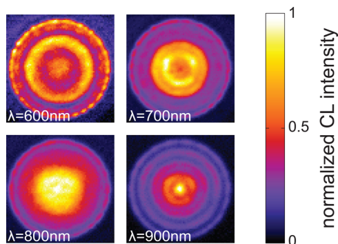
Figure 4. Spatial CL intensity maps of a typical patch antenna with disk diameter of 1.8 \mu\text{m} at four different wavelengths integrated over a bandwidth of 10 nm. CL intensity data are corrected for the background (typically around 100 cts/px/0.25 s) and the system response and are normalized to unity at each wavelength. The maximum counts of the raw map data before correction are equal to 320, 590, 370, and 350 cts/px/0.25 s for wavelengths from 600 to 900 nm, respectively.
