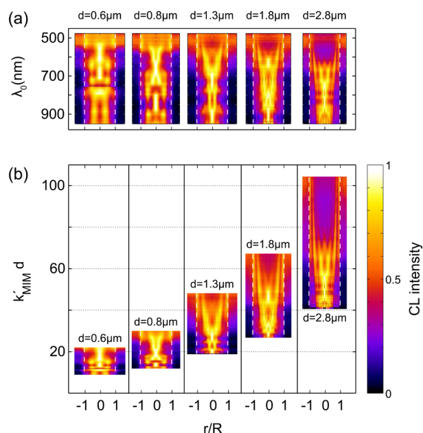
Figure 5. (a) Azimuthally averaged CL intensity maps as a function of wavelength and relative distance to the disk center for five disk sizes: 0.6, 0.8, 1.3, 1.8, and 2.8 \mu\text{m} . (b) CL intensity maps with normalized wavenumber for different disk diameters corresponding to (a). CL intensity data are corrected for the background (typically around 100 cts/px/0.25 s) and the system response and are normalized to unity at each disk size. The maximum counts of the raw map data before correction are equal to 1390, 1030, 990, 630, and 960 cts/px/0.25 s for increasing disk size, respectively.
