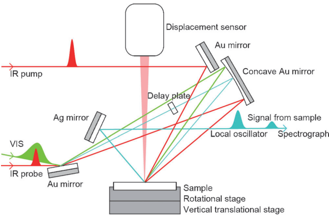
Figure 1. Schematic representation of the 2D-HD-SFG experiments.
