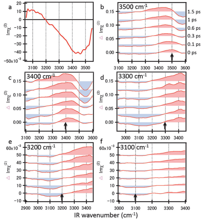
Figure 2. a) Steady-state \text{Im}[\chi^{(2)}] spectrum. b)–f) Time-resolved \Delta\text{Im}[\chi^{(2)}] spectra of the O–H stretching mode at the air/water interface. Waiting times after excitation are 0, 0.1, 0.3, 0.6, 1, and 1.5 ps (from bottom to top). The black arrows indicate the frequency of the pump pulses. Note the different x- and y-scales in panels (b)–(f).
