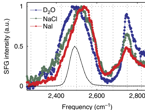
Figure 1 | Static SFG spectra of water and different salt solutions. SFG spectra recorded from the surfaces of 3 M solutions of NaI (red) and NaCl (green) and pure water D 2 O solutions (blue), normalized to the peak SFG intensity. An exemplary spectrum of the excitation pulse around 2500 cm −1 is shown with a thin black line. Dashed lines indicate all the excitation frequencies used in the experiment.
