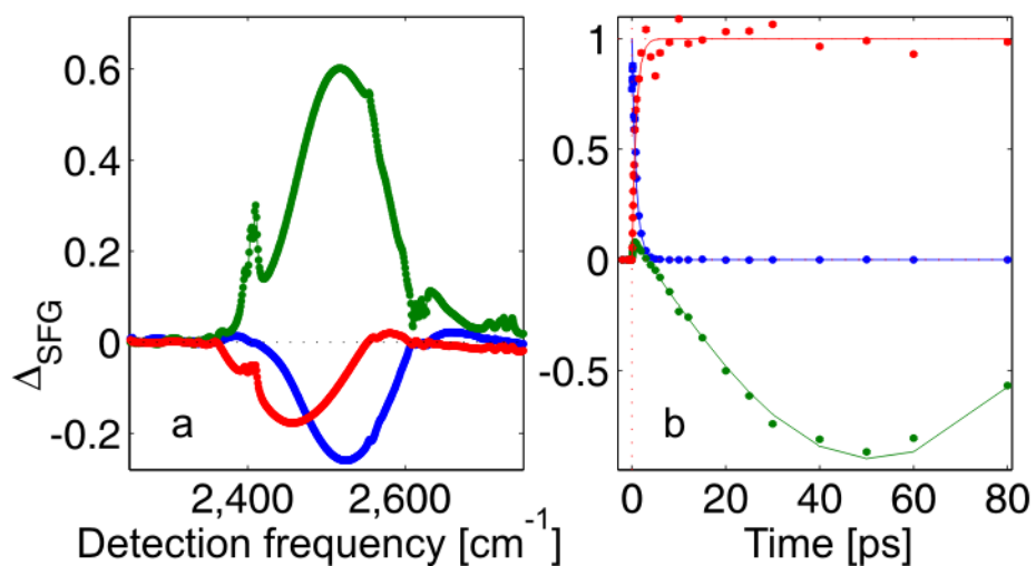
Supplementary Figure 1 Spectral decomposition and population dynamics of the SFG signal. (a) SFG spectra for NaI solution extracted from the global fit to the kinetic model described in the main text. The three spectra correspond to: excited vibrational state (blue), thermally equilibrated state (red) and spectral signature of the oscillatory signal (green). (b) Population dynamics associated with the states included in the model. Solid lines indicate dynamics of the kinetic model. Points indicate time dynamics of the data reconstructed with the extracted spectral signatures.
