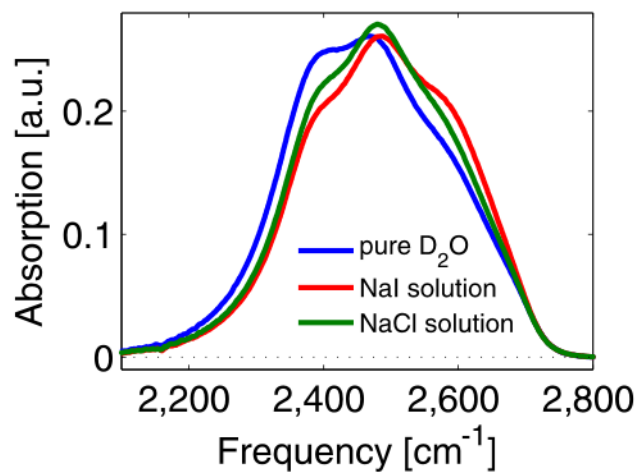
Supplementary Figure 2 Linear absorption spectra of pure D 2 O (blue) and NaI/D 2 O (red) and NaCl/D 2 O (green) solutions. The spectra were recorded with an attenuated total reflectance spectrometer.
