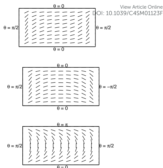
Fig. 1 The diagonal ( D ) state (top), the rotated ( U_1 ) state (middle) and the rotated ( U_2 ) state (bottom), with sample boundary conditions.
