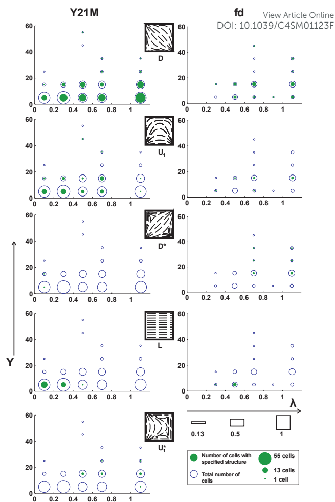
Fig. 6 Phase space for rectangular cells. We plot the length of the shortest side, Y , versus the aspect ratio, \lambda , for the director fields shown in Figure 5. The circle area is proportional to the number of cells. The area of the filled circles is proportional to states exhibiting the specified director field. The left hand column contains results for Y21M and the right hand column for WT fd -virus.
