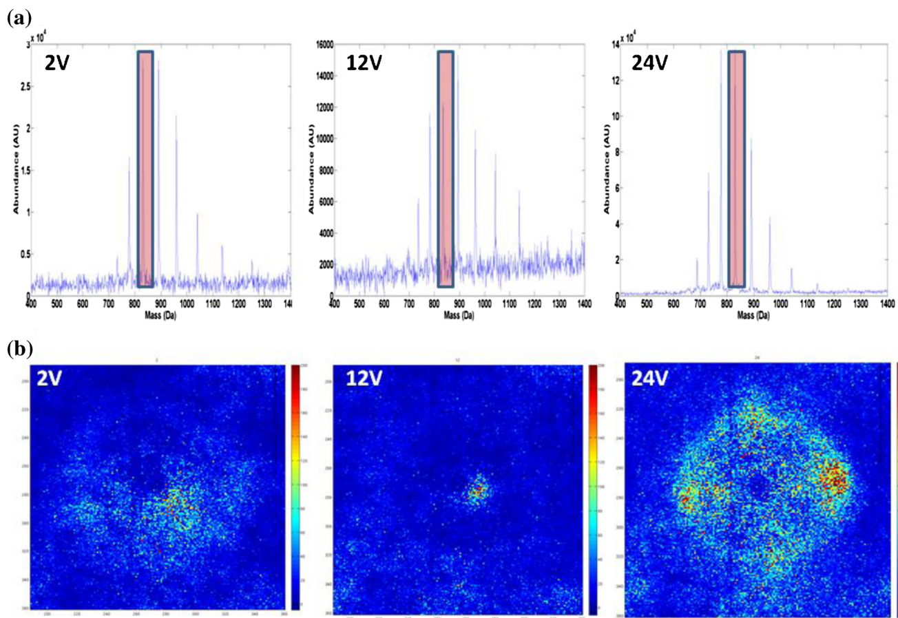
Figure 6. (a) Mass spectrum obtained at three different values of octopole DC bias: 2, 12, and 24 V; (b) corresponding spatial distribution of the peak highlighted in (a), [M + 15H]^{15+}
