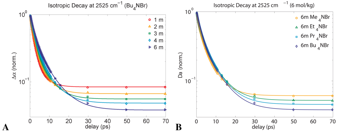
Figure 3. The vibrational decay dynamics becomes slower for increasing concentrations of \text{Bu}_4\text{NBr} (A) and for increasing chain lengths at a concentration of 6\text{ m} (B). The delay traces shown are taken at 2525\text{ cm}^{-1} . The solid lines in the figures are the fit of the kinetic model described in the text to the data.
