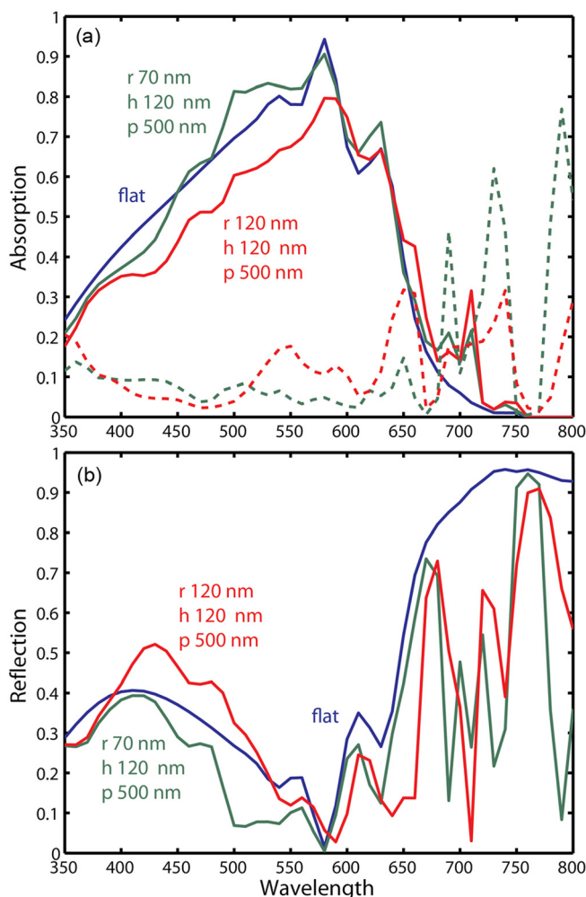
FIG. 4. (a) Simulated absorption in the a-Si:H i -layer (continuous lines) and in the Ag nanoparticles (dashed lines). (b) Simulated reflection from the layer geometry. Data are shown for the experimental nanopatterned cell geometry (red), the flat reference cell (blue), and an optimized design (green).
