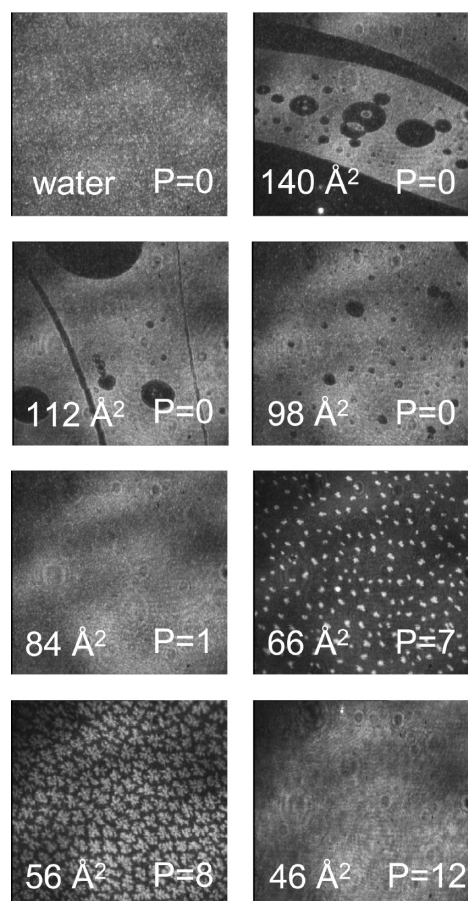
Figure 3. Brewster Angle Microscopy images for different densities of DPPC on water. The image size is 600 \times 600 \mu\text{m} . White regions indicate high density, while black indicates low density. In every panel the area per molecule (in \text{\AA}^2 ) is reported in the bottom left corner and the surface pressure (in \text{mN}/\text{m} ) in the bottom right corner. The pictures are taken with a camera that automatically adjusts its sensitivity, so that the intensity gray scales cannot be compared between images.
