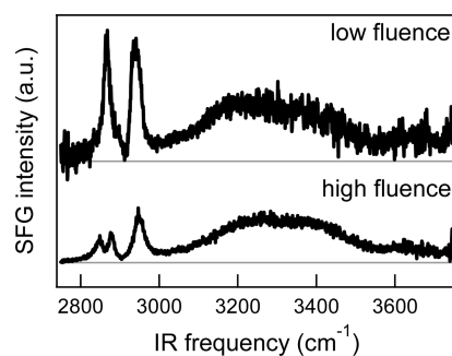
Figure 7. SFG spectra (SSP polarization) for DPPC on water at high density ( \sim 45 \text{ \AA}^2 per molecule) at low ( \sim 1.5 \text{ mJ/cm}^2 ) and high fluence ( \sim 10 \text{ mJ/cm}^2 ), respectively, for which the single pulse heating amounts to between 0.3 and 3 °C (depending on the IR frequency) and between 2 and 19 °C, respectively. The spectra are offset for clarity and are scaled to the relative IR intensities. Note the very different shape, as a result of thermal effects occurring at high fluence. Both spectra were measured with a nonrotating trough.
