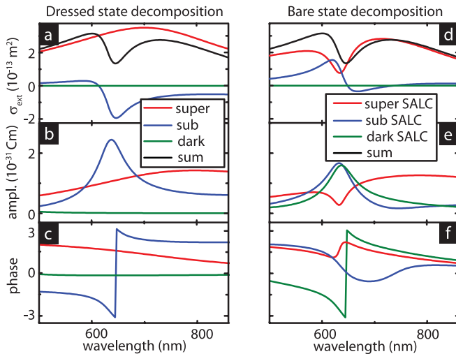
FIG. 4 (color). (a) Calculated contribution of eigenmodes [Fig. 3(b)] to extinction cross section of plasmonic heptamers. (b) Eigenmode amplitude and (c) phase relative to driving field. (d), (e), (f) Corresponding graphs in the nondiagonal bare state basis [Fig. 3(a)].
