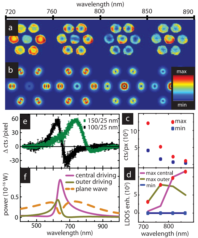
FIG. 2 (color). (a) Measured CL excitability maps of plasmonic heptamer. (b) Calculated maps of radiative LDOS. Insert: colorbar for (a) and (b). (c) Limits of color scale for (a). Background around 700 nm stems from oxide substrate. (d) Calculated radiative LDOS enhancement on central (purple) and outer (olive) particles of heptamer with particle diameter/gapwidth 150/25 nm. Blue and red symbols denote color scale limits of frames in (b). (e) Measured differential excitability spectra showing intensity difference between outer and central particles. Green (black): Particle diameter/gap width 150/25 nm (100/25 nm). Error bars denote standard deviation of 4 (2) structures. (f) Calculated power radiated by super- and sub-radiant eigenmodes of heptamer upon driving central (purple)/outer (olive)/all (orange dashed) particles with vertical electric field, corresponding to black curve in (e) (100/25 nm).
