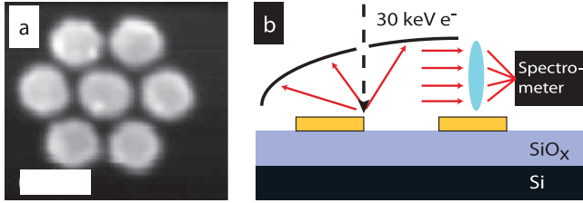
FIG. 1 (color). (a) SEM micrograph of plasmonic heptamer. Scale bar is 200 nm. (b) Sketch of experimental setup showing sample, impinging electron beam, parabolic mirror, and optics guiding CL to a spectrometer.
