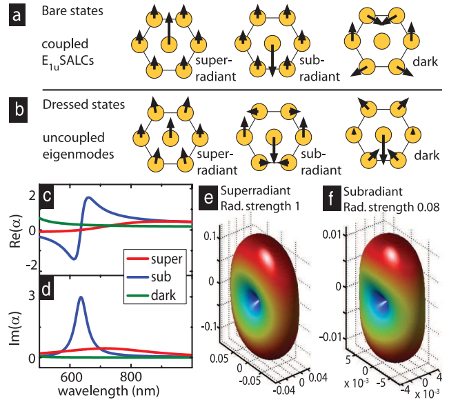
FIG. 3 (color). (a) Bare state nondiagonal polarization basis, consisting of a superradiant, subradiant and dark SALC of E_{1u} derived from group theory. (b) Dressed state basis of decoupled superradiant, subradiant, and dark eigenmodes (small out-of-phase components not visualized). (c) Real and (d) imaginary parts of polarizabilities of the eigenmodes in 10^{-31} \text{Cm}^2/\text{V} . (e) and (f) are radiation patterns of superradiant and subradiant eigenmodes in \text{W}/\text{sr} . Radiative strength indicates total radiated power relative to the superradiant eigenmode.
