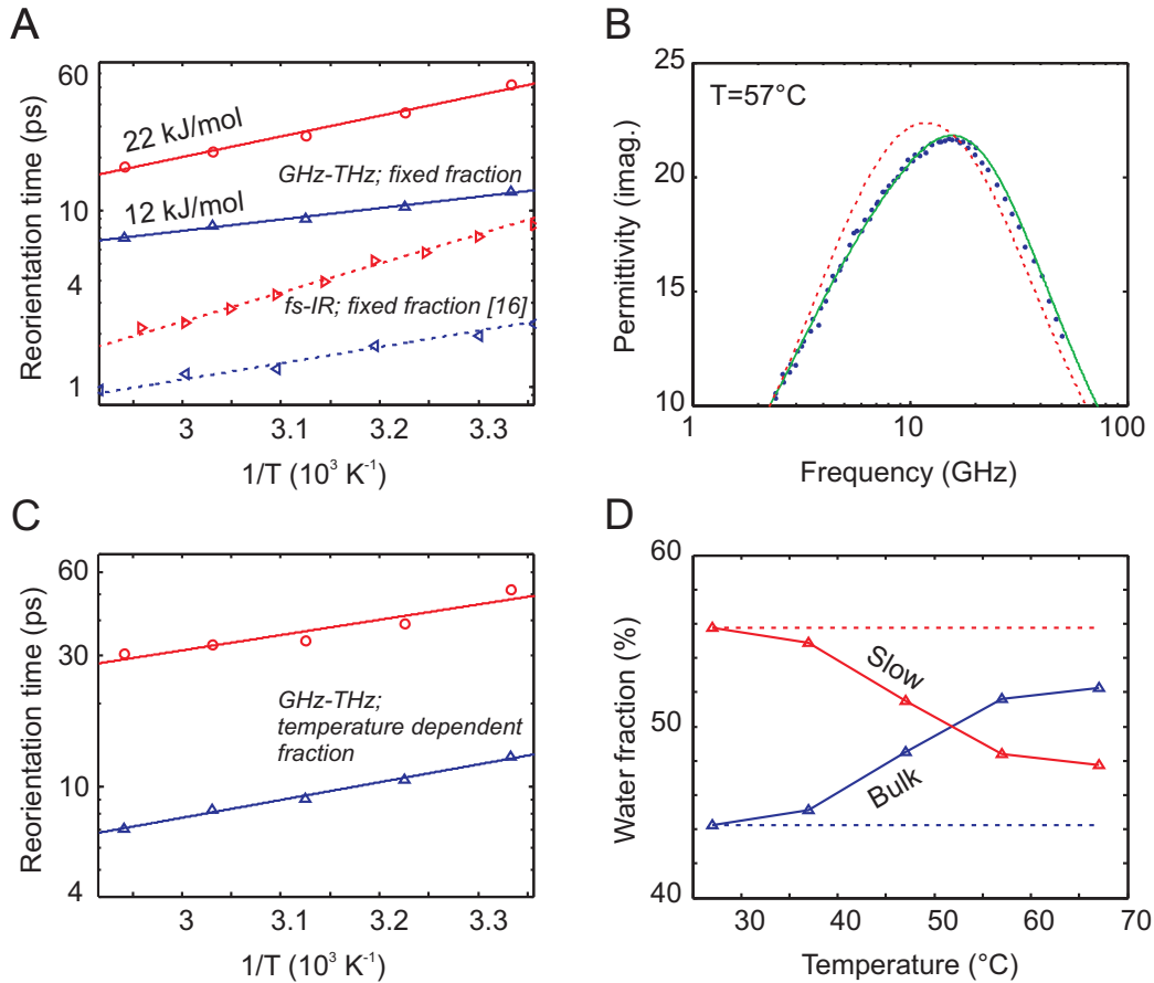
Figure 6: A The fit results when the fractions of bulk-like and slow water are fixed for the GHz-THz measurements ( \circ, \triangle ), together with fs-IR measurements ( \triangleright, \triangleleft ) from Ref. [16], where the same assumption was made. B A comparison of the fit for TMU w = 0.07 at 57^\circ\text{C} , where the fraction of bulk-like is free (line) and where it is kept constant over temperature (dotted line). C The reorientation time for bulk-like water (circles) and TMU/slow water (triangles) as a function of 1/T with fits where the water fractions were free. Note that the slope of the slow water species in this case does not represent the activation energy of the hydrophobic hydration shell water, as the number of water molecules in this ensemble is not constant with temperature. D The fraction of bulk-like water as function of temperature ( \triangle ) and the fixed fraction of bulk-like water for the alternative fit (dotted line).
