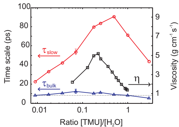
Figure 3: The extracted reorientation time scale for the slow hydration shell water \tau_{\text{slow}}(c) ( \circ ), the reorientation time scale for bulk-like water \tau_{\text{bulk}}(c) ( \triangle ), and the viscosity ( \square ; data from Ref. [30]) as a function of TMU concentration. The dashed line represents the reorientation time for bulk water \tau_{\text{bulk}}(0) . Error bars are given as an indication.
