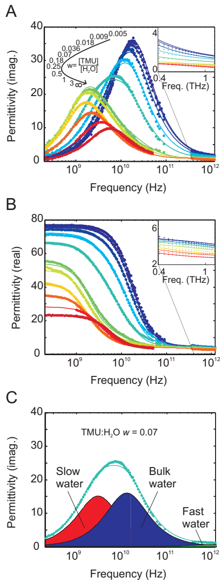
Figure 1: Combined data (dots) and fits (lines) from GHz and THz dielectric relaxation spectroscopy, showing the imaginary ( \epsilon'' ) (A) and real ( \epsilon' ) (B) permittivity as a function of frequency for different TMU concentrations, given in ratios of TMU:H 2 O. The insets show the frequency dependence in the THz regime more closely. C A decomposition into the three dielectric relaxation processes (slow hydration shell water, bulk-like water and fast water) for w = 0.07 .
