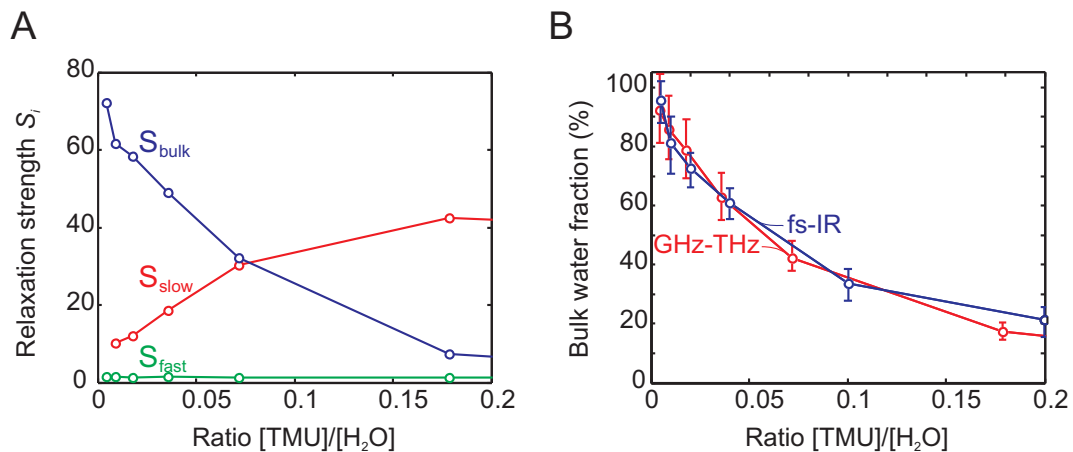
Figure 2: A The extracted relaxation strengths S_i for the slow component, the bulk-like water and the fast water. B The extracted fraction of bulk-like water, based on the fits to the GHz-THz data and the fs-IR data, as a function of TMU concentration.
