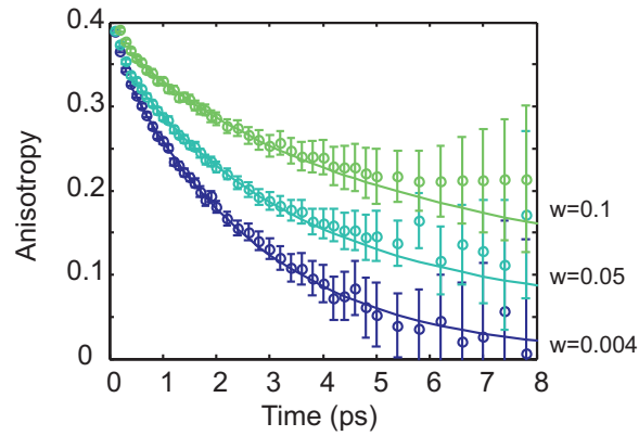
Figure 4: The anisotropy decay as a function of pump-probe delay time for a number of TMU concentrations, from Ref. [13]. To describe these data (lines), the resulting time scales from the GHz-THz measurements \tau_{\text{slow}}(c) and \tau_{\text{bulk}}(0) were used, after correction for the difference between macroscopic first order (GHz-THz) and microscopic second order (fs-IR) correlation function measurements.
