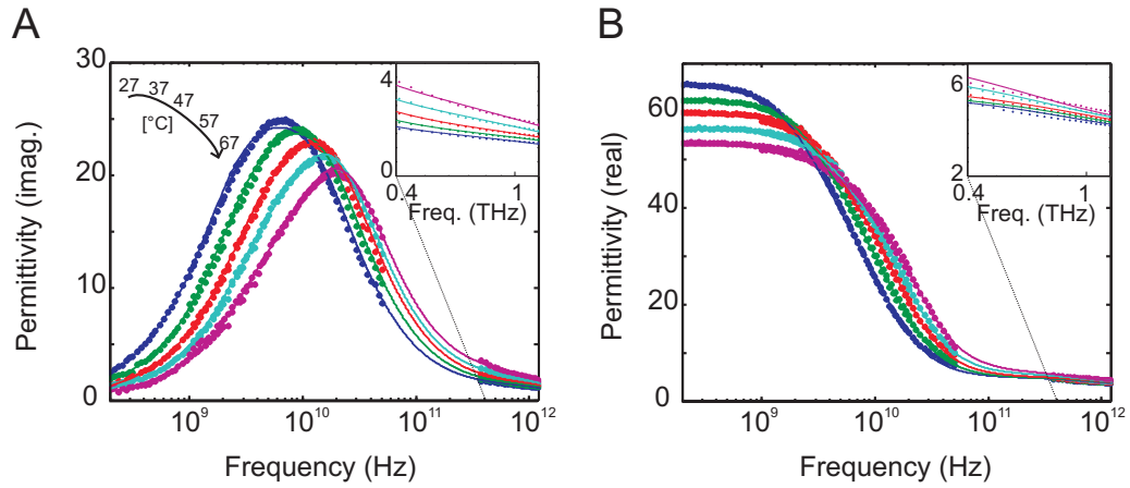
Figure 5: The imaginary (A) and real (B) part of the permittivity for a solution of TMU in water (4 mol/kg) at different temperatures. The insets show the frequency dependence in the THz regime more closely .
