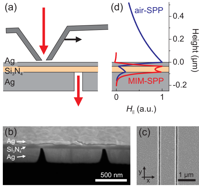
Figure 1. (a) Schematic depiction of the measurement geometry. Laser light is incident through the aperture of an Al near-field probe, which is scanned with respect to the sample. Light transported through the MIM waveguide is collected after scattering from subwavelength slits in the back Ag film. (b, c) SEM micrographs of the fabricated waveguide, shown in cross-section (b) and as viewed from the bottom (c). The waveguide consists of 50 nm of \text{Si}_3\text{N}_4 clad with 35 nm Ag on the top and 310 nm Ag on the bottom. (d) H field mode profiles of the two waveguided SPP modes supported by the multilayer stack.
