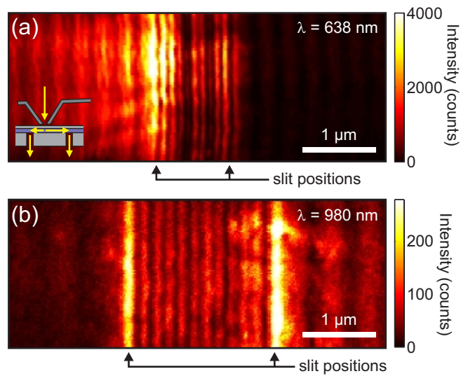
Figure 3. (a) Near-field image obtained by scanning the excitation tip position over the sample containing a pair of output slits separated by 1 \mu\text{m} . Excitation wavelength is 638 \text{ nm} . The inset shows the interference mechanism leading to the fast spatial intensity oscillations between the slit. (b) Near-field image as in (a), but for an excitation wavelength of 980 \text{ nm} and a slit separation of 2 \mu\text{m} .
