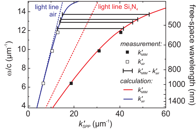
Figure 4. Dispersion relations of the two SPP modes that are supported by the system. Closed and open symbols indicate the measured values of k'_{MIM} and k'_{air} , respectively. The length of the horizontal bars at high frequencies is equal to the experimentally-determined values of (k'_{MIM} - k'_{air}) . The solid blue and red lines are the calculated dispersion curves for the air and MIM-SPP modes, respectively.
