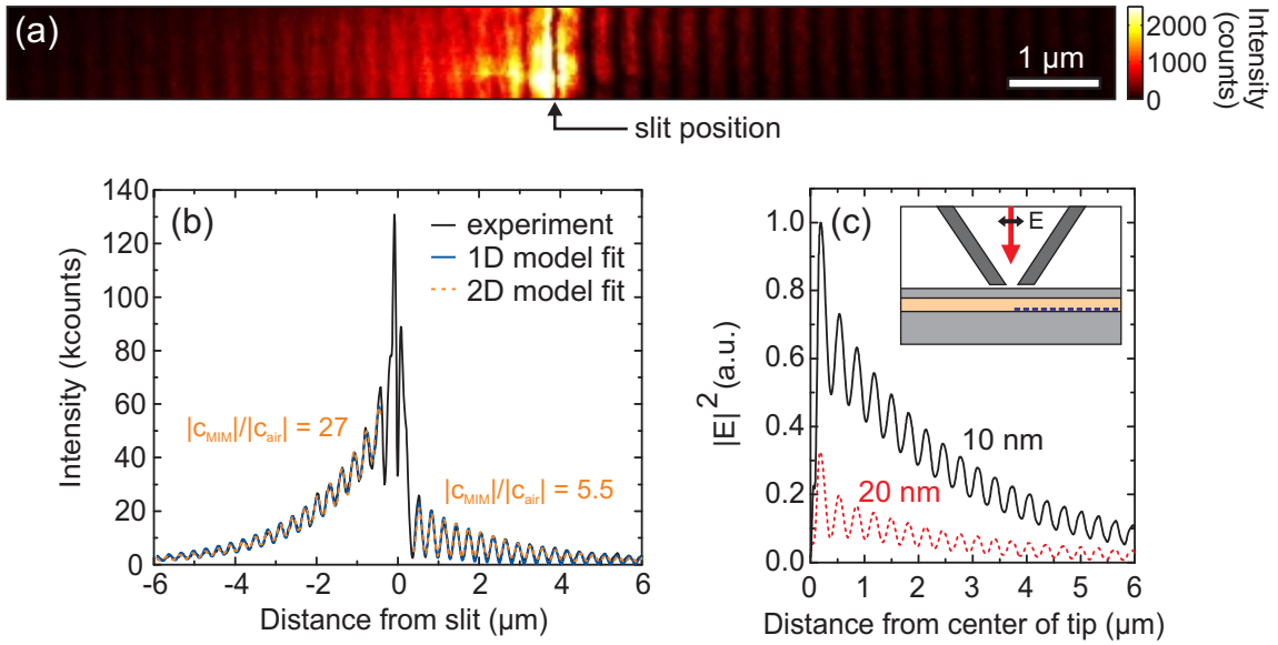
Figure 2. (a) Near-field image obtained by scanning the excitation tip position over the sample containing a single output slit. The excitation wavelength is 638 nm. (b) Collected intensity in Fig. 2(a) as a function of tip-slit distance (black curve), and a fit to the data of the one- and two-dimensional models described in the text (blue and orange curves, respectively). The ratio of the amplitudes of both modes in the 2D model is indicated. (c) Simulated electric field intensity in the \text{Si}_3\text{N}_4 film as a function of distance from the center of the tip. The inset shows a schematic of the simulated two-dimensional geometry. The dashed blue line indicates the position at which the calculated intensity is plotted. The tip-sample separation is 10 nm (black) or 20 nm (red).
