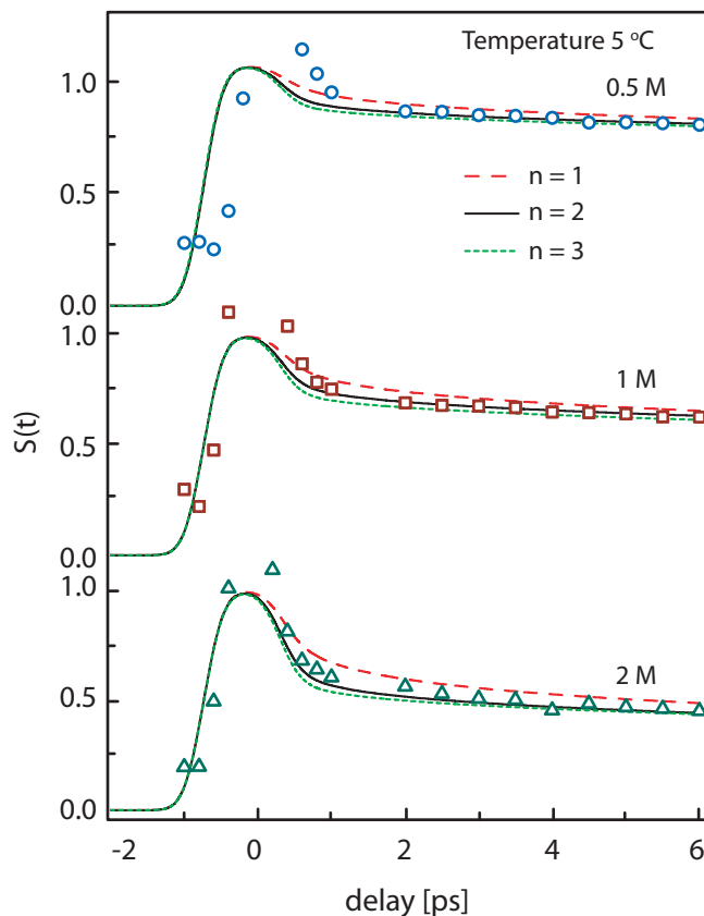
Figure 4: The data from Figure 3, on a linear scale and up to 6 ps, is compared with the theoretical solution which is convoluted with an IRF of 500 fs FWHM. The values of D used in the calculation are given in Table 1. For n = 2 (full lines) the values of \sigma are collected in Table 2 (see eq 2). The best fits for n = 1 and 3 are shown by the dashed lines. The values of \sigma for n = 1 are 0.44, 0.4, and 0.37 Å for c = 0.5, 1, and 2 M, respectively, while for n = 3 they are 5.0, 3.7, and 3.0 Å 3 .
