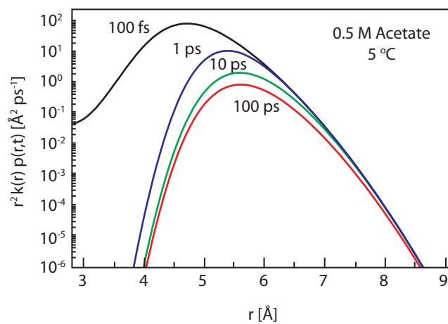
Figure 9: The distance dependence of the radial reactive flux density for PT between HPTS* and 0.5 M acetate at 5 °C, with \sigma = 1.5 \text{ Å}^2 (Table 2).
