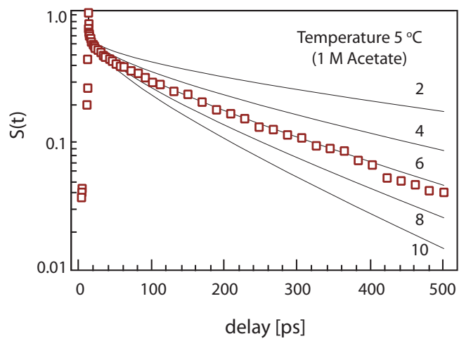
Figure 5: The effect of varying the diffusion constant on the acid-base kinetics, demonstrated for the reaction of HPTS* with 1.0 M acetate at 5° C (same data as in Figure 3). The lines were calculated with \sigma = 1.2 \text{ \AA}^2 (see Table 2) and the indicated values of D (in units of 10^{-6} \text{ cm}^2/\text{s} ).
