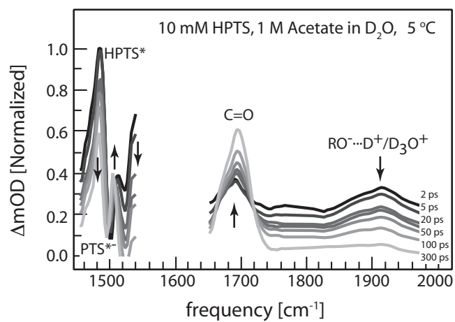
Figure 1: Transient mid-IR absorption spectra of 10 mM HPTS in liquid D 2 O solution containing 1 M of sodium acetate at 5 °C and different delay times following the exciting 400 nm pulse.
