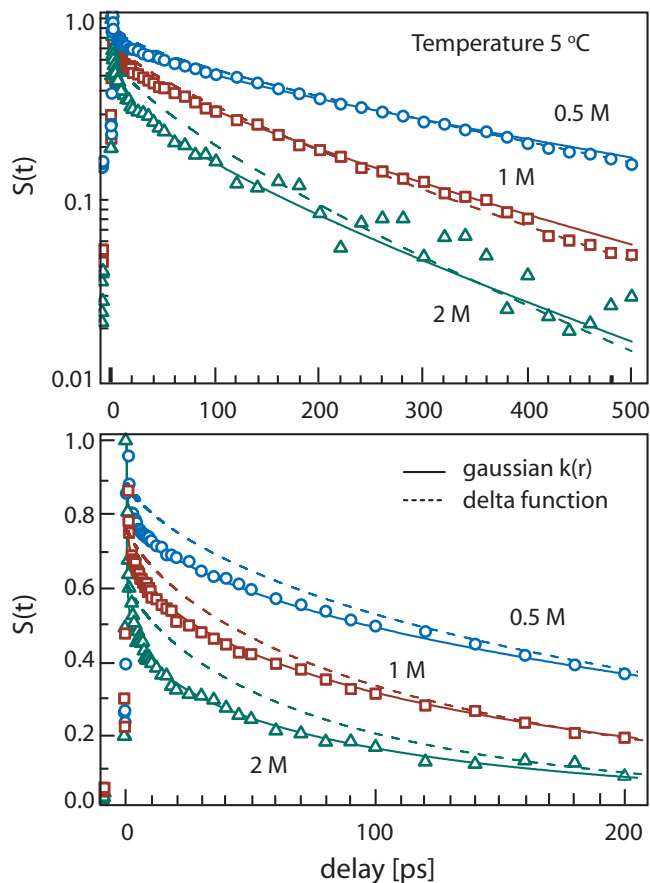
Figure 3: Time resolved IR signals (symbols) from excited HPTS in D_2O at 5^\circ C and three acetate concentrations, normalized at 1 ps (to 0.89, 0.76, and 0.61 for c = 0.5 , 1, and 2 M acetate, respectively), are depicted as symbols on two different timescales: (a) semi-logarithmic (up to 500 ps), and (b) linear (up to 200 ps). Dashed/full lines are fits to the solution of eqs 5–7 with two different sink terms: (i) Delta-function sink (dashed lines), eq 8, with a = 6.8 \text{ \AA} and k_0 = 100 , 60, and 35 \text{ ns}^{-1} for c = 0.5 , 1, and 2 M acetate, respectively. (ii) Gaussian sink term, eq 2 with n = 2 , and parameters in Tables 1 and 2 (full lines).
