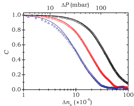
FIG. 2: RIT autocorrelation coefficient as a function of \Delta n_h . Data points show measurement results for 3 slabs of polyethylene filters ( L = 1, 1.5, and 2 mm for black squares, red circles, and blue triangles, consequently). The lines show the fit to theory (Eq. (5)).
