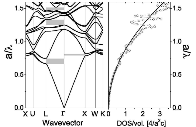
Fig. 6. Left : Photonic band structure (Media 2) for the \text{TiO}_2 inverse opal shown in Fig. 5. The grey rectangles indicate stopgaps in the \Gamma\text{L} direction and one stopgap in the \Gamma\text{X} direction for the inverse opal. The stopgaps result in the decreased DOS ( right : circles, Media 3) at corresponding frequencies compared to the DOS in a homogeneous medium with n_{av} = 1.27 ( right : solid line).
