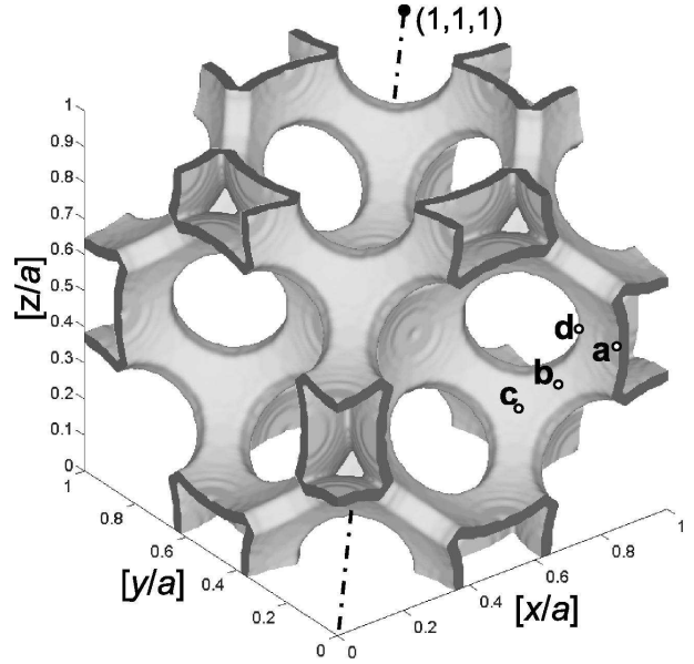
Fig. 5. Rendering of the dielectric function in one fcc unit cell that models the \text{TiO}_2 inverse-opal structure in section 4: an fcc lattice of air spheres of radius r = 0.25\sqrt{2}a with a being the cubic lattice parameter. The spheres are covered by shells with \epsilon = 6.5 and outer radius 1.09r . Neighboring air spheres are connected by windows of radius 0.4r . The letters (a-d) indicate four different positions at the \text{TiO}_2 -air: a = (1, 0, 0)/(2\sqrt{2}) , b = (1, 1, 2)/(4\sqrt{3}) , c = (1, 1, 1)/(2\sqrt{6}) and d = (0.33, 0.13, 0) (points shown are symmetry-equivalents). The dash-dotted line shows the main diagonal of the cubic unit cell.
