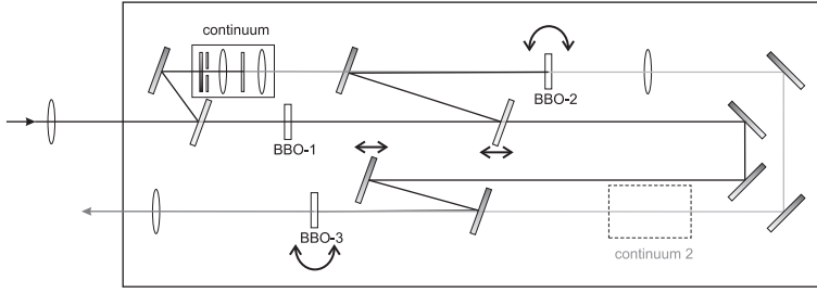
FIGURE 2.8. Schematic representation of the NOPA. The incoming beam is weakly focused and split in two. Subsequently one part enters the first continuum stage. The other part is frequency doubled in the BBO-1 crystal and split again after which one part is overlapped with the continuum in the BBO-2 crystal. The newly formed beam is sent to BBO-3 crystal, where it is overlapped with the remainder of the frequency doubled beam, to be amplified. Optionally a second continuum stage can be entered to generate wavelengths around 800 nm.
