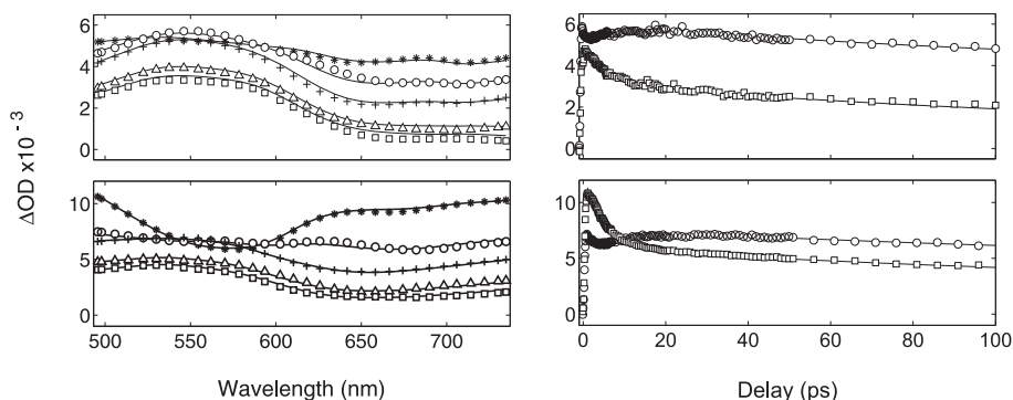
FIGURE 8.10. [Left] Transient absorption spectra of the switch in the open (top) and closed form (bottom) at 2 (stars), 10 (circles), 50 (crossed), 250 (triangles) and 550 ps (squares). [Right] Transient kinetics of switch in the open (top) and closed form (bottom) at 550 (circles) and 750 nm (squares). Excitation wavelength 266 nm, 300 nJ/pulse. The symbols represent the data, the lines are results of the global fits.
