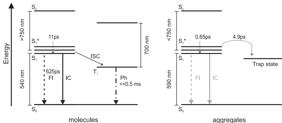
FIGURE 7.8. Energy diagram for 1o in the form of isolated molecules (left) and aggregates (right). At room temperature only isolated molecules are present, while aggregation is observed at lower temperatures. At low temperatures there is a mixture of a (minor fraction of) isolated molecules and of the aggregates. Therefore, at 125 K both energy level diagrams are relevant and a combination of time constants, long for the isolated molecules and short for the aggregates, and spectral features belonging to both cases can be expected in the transient absorption experiments at low temperatures
