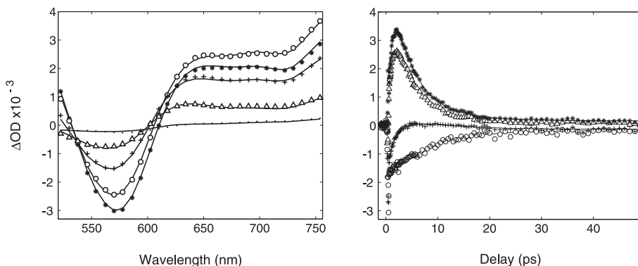
FIGURE 9.22. [Left] Transient spectra of CSC in the closed form at 1 (stars), 2 (circles), 5 (crosses), 10 (triangles) and 50 ps (dots). [Right] Transient kinetics of CSC in the closed form at 550 (circles), 600 (crosses), 700 (triangles) and 750 nm (stars). Excitation wavelength 550 nm, 420 nJ/pulse. The symbols represent the data, the lines are results of the global fits.
