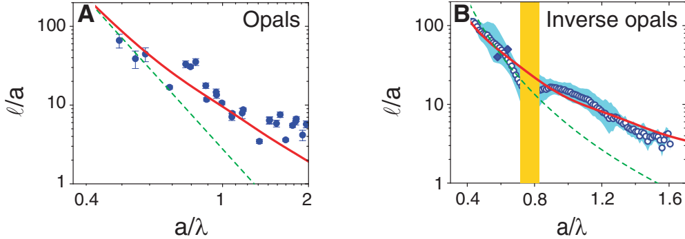
FIG. 2: (color) Symbols: mean free path [14] \ell in units of a versus normalized frequency a/\lambda in polystyrene opals (A) and titania inverse opals (B). Open symbols in (B) were obtained by averaging for each a/\lambda total transmission spectra for many samples with different a . The blue shaded area indicates the standard deviation. In the stop gap (orange bar), total transmission is reduced in excess of \ell/L due to Bragg reflection of the input beam. This affects the data in this limited range. Previous data show that \ell is unaffected if the frequency is tuned through a gap [16]. In both (A) and (B), the extinction length agrees well with the model (1,2) with \delta R \sim 5\% (red curves). Green curves represent scaling of \ell with \omega^{-4} , and illustrate the failure of Rayleigh scattering models.
