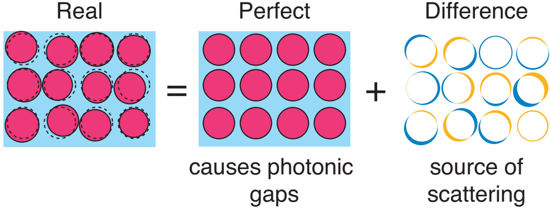
FIG. 1: (Schematic) Any 2D or 3D real photonic crystal is an ordered stack of building blocks with a spread \Delta r in their average radius r , each slightly displaced (displacement \Delta u ) from the lattice sites. The real structure is the sum of the perfect crystal and the difference between the real and perfect structure. This difference is a collection of thin shells that each scatter weakly. Due to their high number density, the shells dominate the scattering loss.
