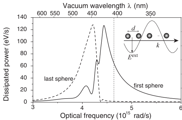
FIG. 1: Excitation by a plane wave along the array causes a localized optical response in finite plasmon arrays (10 Ag particles in glass, radius 30 nm, d = 75 nm). Depending on driving frequency, the Ohmic dissipated power (at 1 V/m incident field) is either concentrated on the first (solid curve), or last sphere (dashed) encountered by the incident beam. Vertical dashes indicate the single particle resonance frequency.
