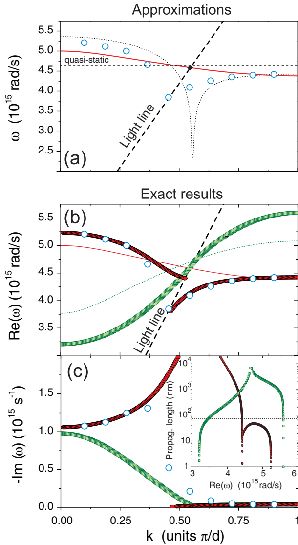
FIG. 2: (Color online) (A) The quasistatic dispersion (solid red curve) for transverse modes intersects the light line (dashed) slightly below the single particle resonance (horizontal dashes). Blue open circles show the 10 normal mode frequencies for an array of 10 particles, according to Ref. [7], which agree neither with the quasistatic dispersion, nor with the perturbative result of Ref. [8] (dotted curve). (B) Red solid circles (green open squares): real part of the frequency for roots of the exact infinite chain dispersion for transverse (longitudinal) modes. For transverse modes two branches appear that anticross at the light line (dashed). The result agrees well with the finite array dispersion (blue open circles taken from (A)), but not with the quasistatic approximation (thin curves, dotted for longitudinal mode). (C) Imaginary part of the frequency for the modes in (B). The damping rate diverges near the light line for transverse modes. Inset in (C): Propagation lengths (amplitude 1/e lengths) versus frequency for transverse (red solid circles) and longitudinal modes (green open squares). The horizontal dashed line indicates the inter-particle spacing d .
