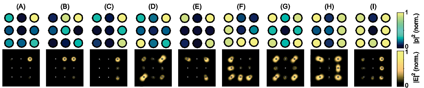
Figure 4. (Color) For a mask containing a 3 by 3 array of Ag particles (spacing 75 nm) 9 out of 138 conceivable combinations of particles can be addressed individually. Other configurations can only be exposed sequentially. The filled dots show the relative amount of excitation on each sphere (grayscale); the contour plots show the resulting electric field intensity in a plane just 5 nm above the mask.
