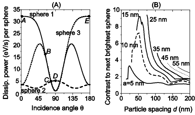
Figure 2. (A) We consider the dissipated power per sphere (at 1V/cm incident field) for nanospheres in a linear array of 3 silver particles ( a=25 nm radius, d=75 nm spacing in glass ( n=1.5 )) illuminated with a 500 nm wavelength plane wave incident and polarized in the \varphi=0 plane. The spheres are located on the x -axis (coordinate system defined in Fig. 1). As the incident angle \theta is scanned, the distribution of power over the spheres changes (solid line: sphere 1 at x=-d ) furthest from the incident direction at \theta=0 ; dashed line: middle sphere (sphere 2 at x=0 ); dotted line: sphere 3 at x=d closest to the incident beam at \theta=0 ) and allows different exposure patterns. For \theta=0 and 180^\circ , power localizes on a single end sphere. (B) Contrast of the end sphere relative to the next brightest nanoparticle, as a function of particle spacing for different particle radii a as labelled. For each particle spacing the wavelength was optimized and \theta was kept at 0 for optimum contrast of the end particle. For spacings in the range from 25 to 150 nm a useful contrast for programmable plasmon lithography is obtained.
