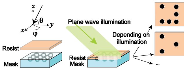
Figure 1. (Color) We consider a transparent mask (refractive index 1.5) containing a configuration of closely spaced silver nanoparticles. Resist is pressed onto this mask, and illuminated using unfocused light. A high field intensity, and hence an exposure in the resist, is created on certain combinations of particles. Which combinations are addressed can be controlled by the wavelength, polarization and incidence angle of the incident light. The upper left inset shows the coordinate system used throughout this work. The mask is in the xy plane. The incident direction is specified by the polar angle \theta relative to the mask normal, and the angle \phi in the plane of the resist.
