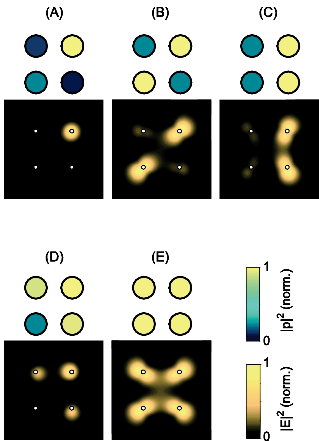
Figure 3. (Color) For a mask containing a 2 by 2 array of Ag particles (spacing 75 nm) all conceivable combinations of particles can be addressed individually. The filled-in dots show the relative amount of excitation on each sphere (grayscale); the contour plots show the resulting electric field intensity in a plane just 5 nm above the mask; the location of the spheres is indicated by open circles. Incidence conditions are listed in the text.
